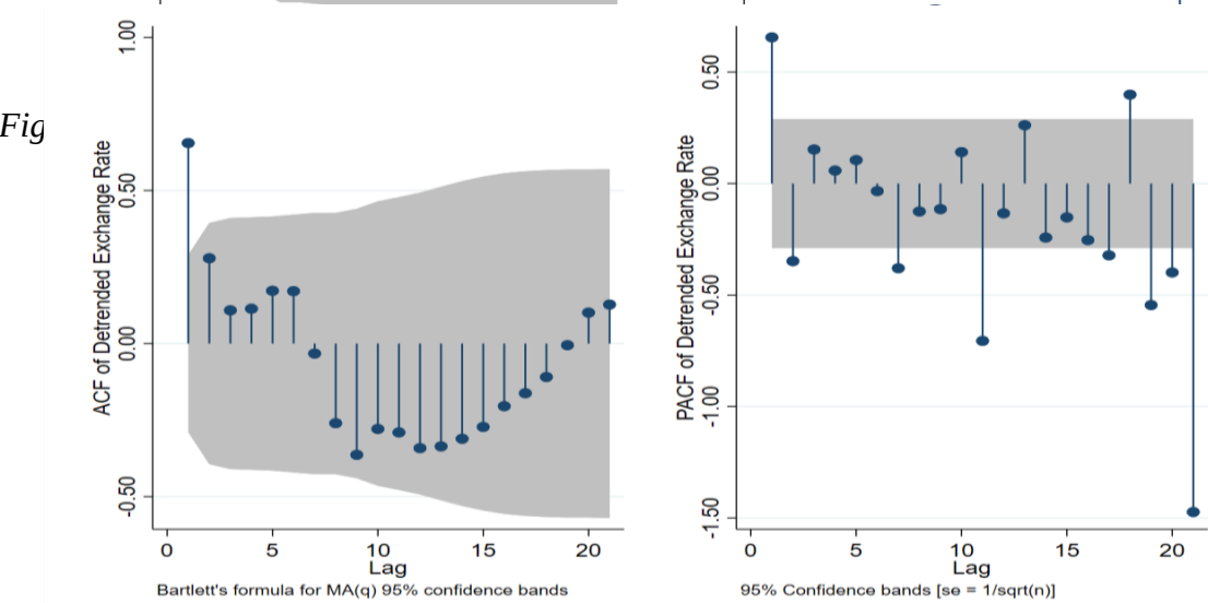
Figure C.3: ACF and PACF of Detrended Exchange Rate
