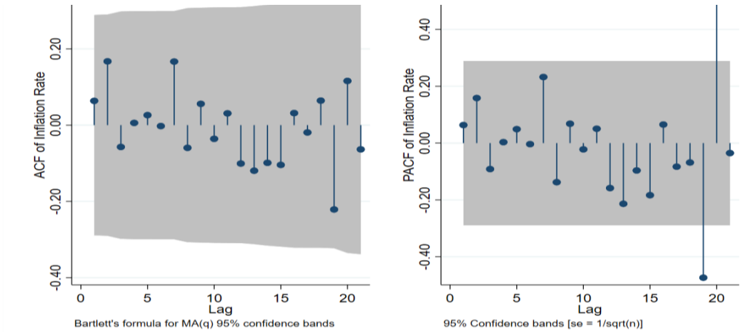
Figure C.4: ACF and PACF of Inflation Rate
