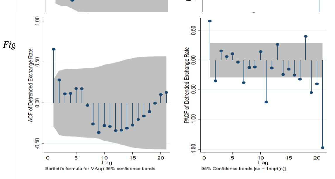
Figure C.3: ACF and PACF of Detrended Exchange Rate
