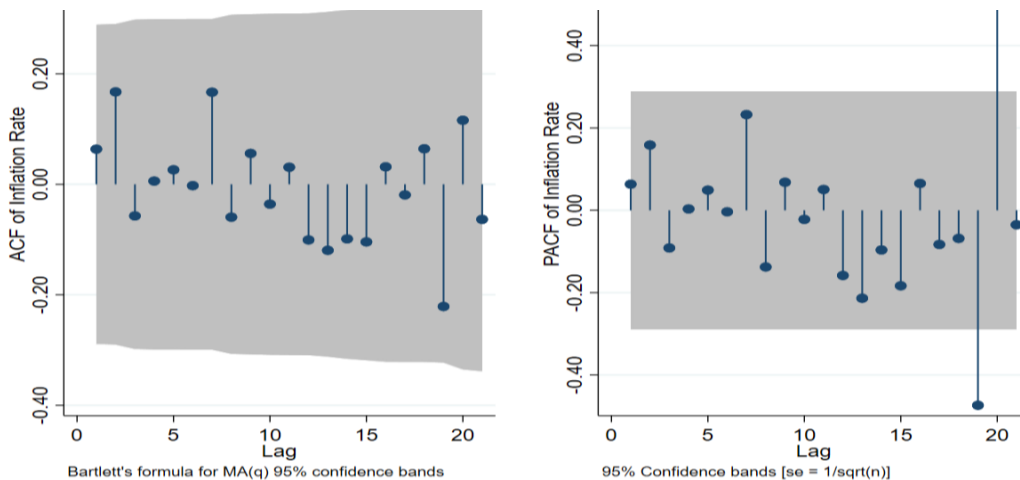
Figure C.4: ACF and PACF of Inflation Rate
